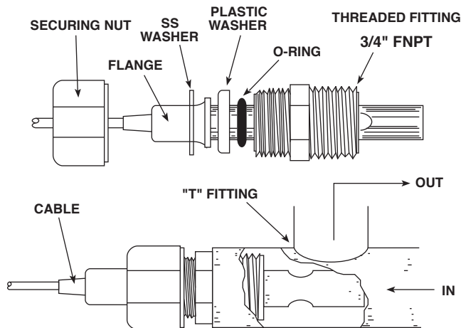
INSERTION MODE ASSEMBLY
