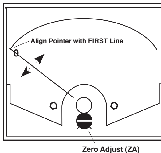
CLEAR PLASTIC COVER (case not shown for clarity) Figure II.G.9
