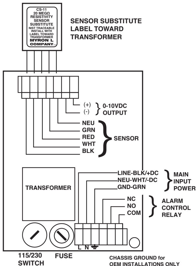
ELECTRICAL CONNECT DIAGRAM
