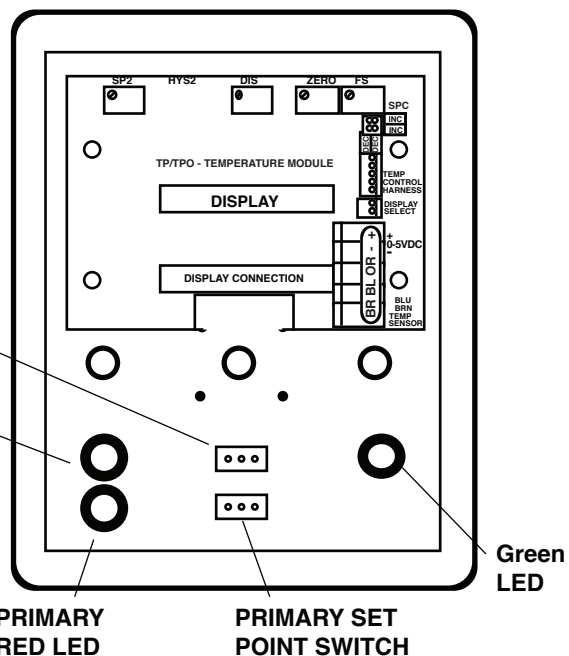
FRONT PANEL Rear View
