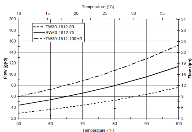
Figure 3: Impact of temperature on permeate flow (constant pressure, recovery)
